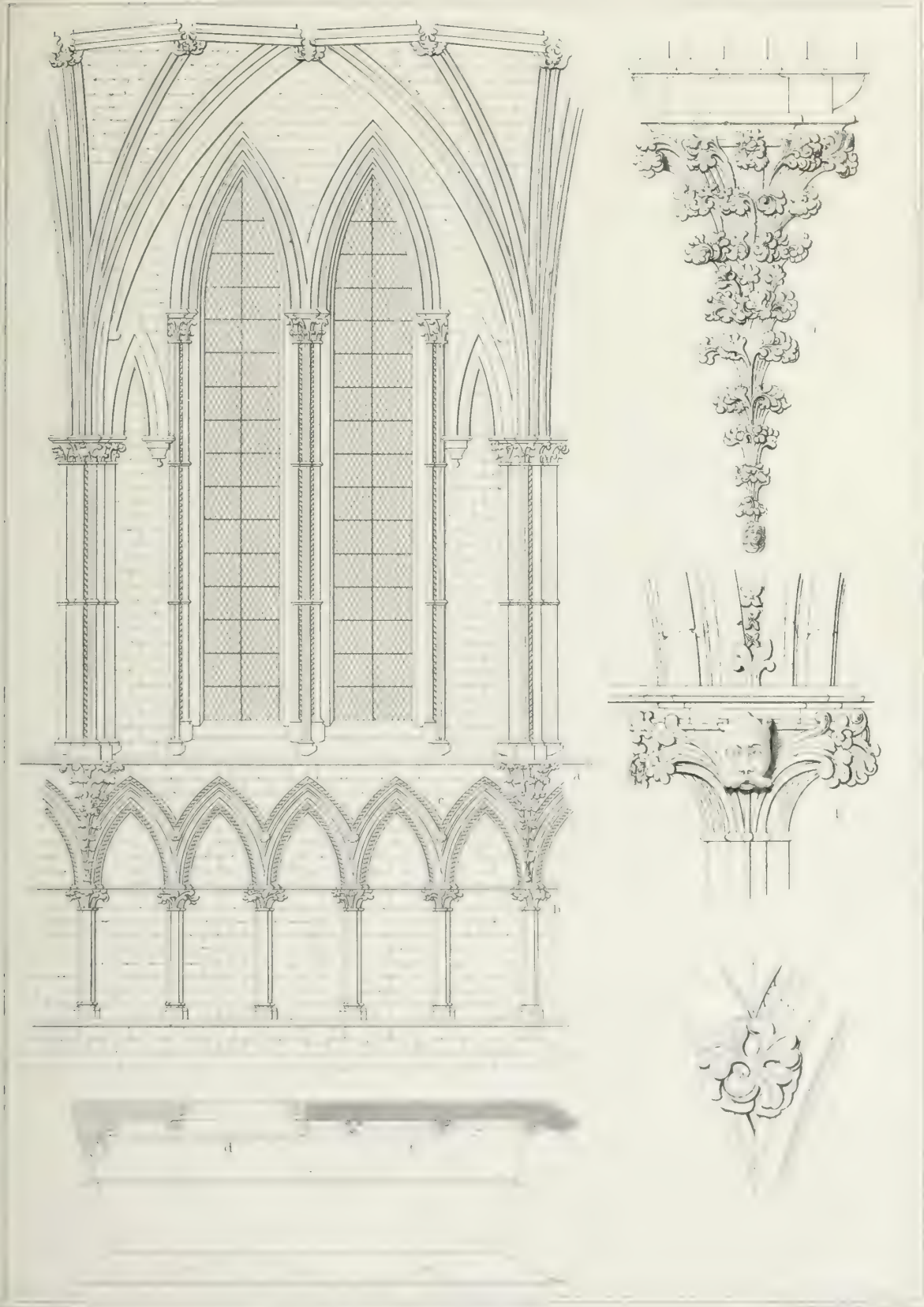
THE GREAT CHURCH OF NOTRE-DAME DE PARIS. ELEVATION OF THE WEST WINDOW. ELEVATION OF THE GALLERY. DETAILS OF CAPITALS AND ARCHES.
